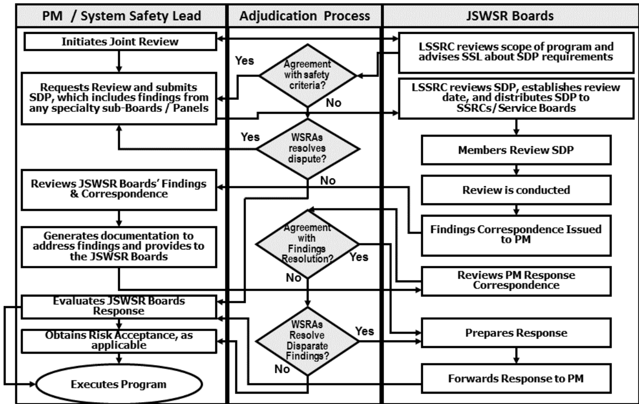
Figure 1. JSWSR Process
