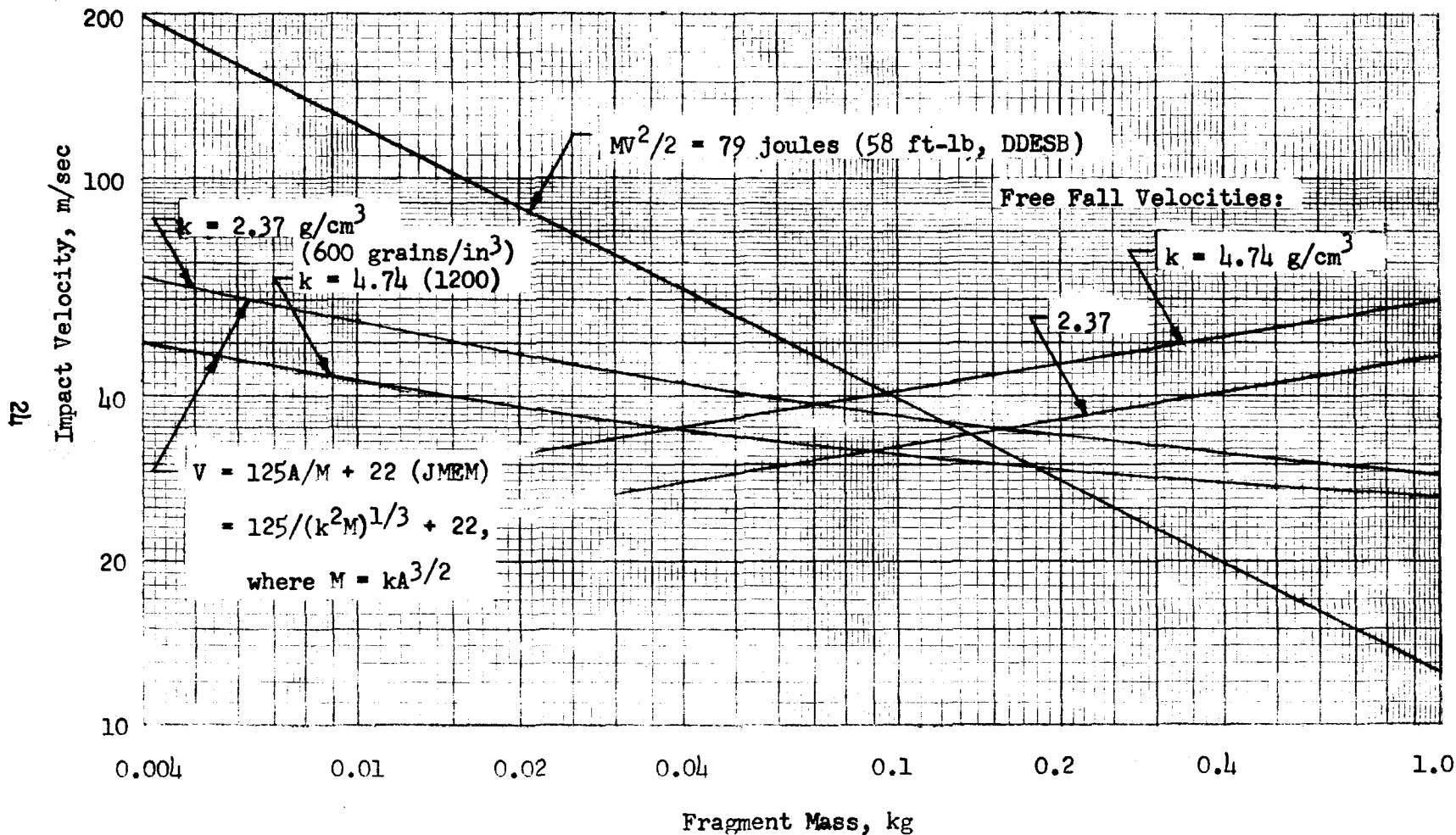
Figure 4 Mass-Velocity Relationships for Fragments
