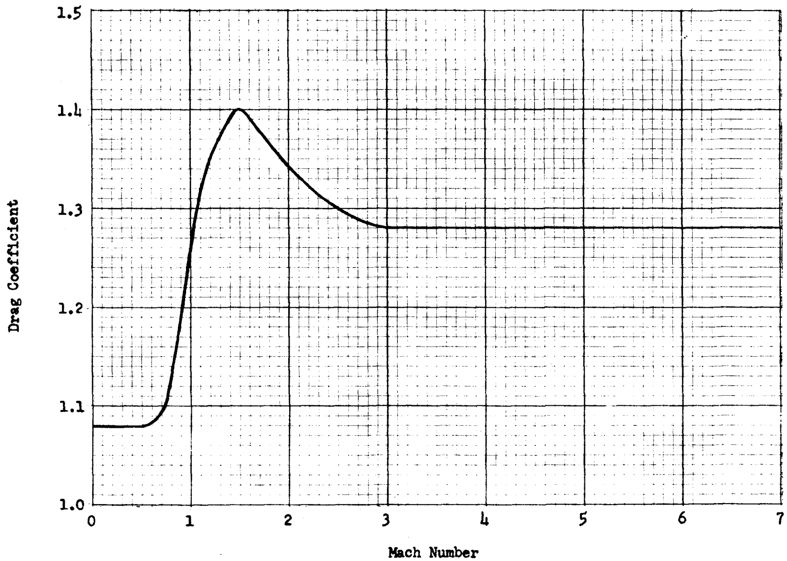
Figure 3 Drag Coefficient of Fragments
