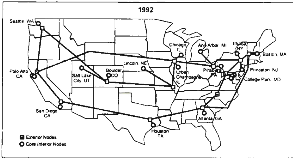
Exhibit 2-5 1992 T3 NSFNET Backbone
