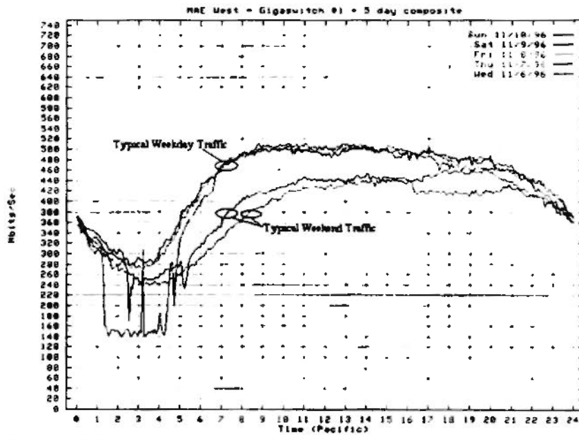
Exhibit 4-8 Typical Traffic Patterns at MAE-WEST
