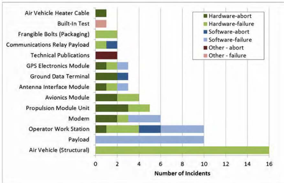
Figure 4-2. Failure chargeability
