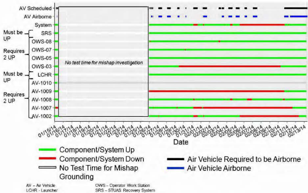
Figure 4-4. RQ-21A System Availability at Twentynine Palms
